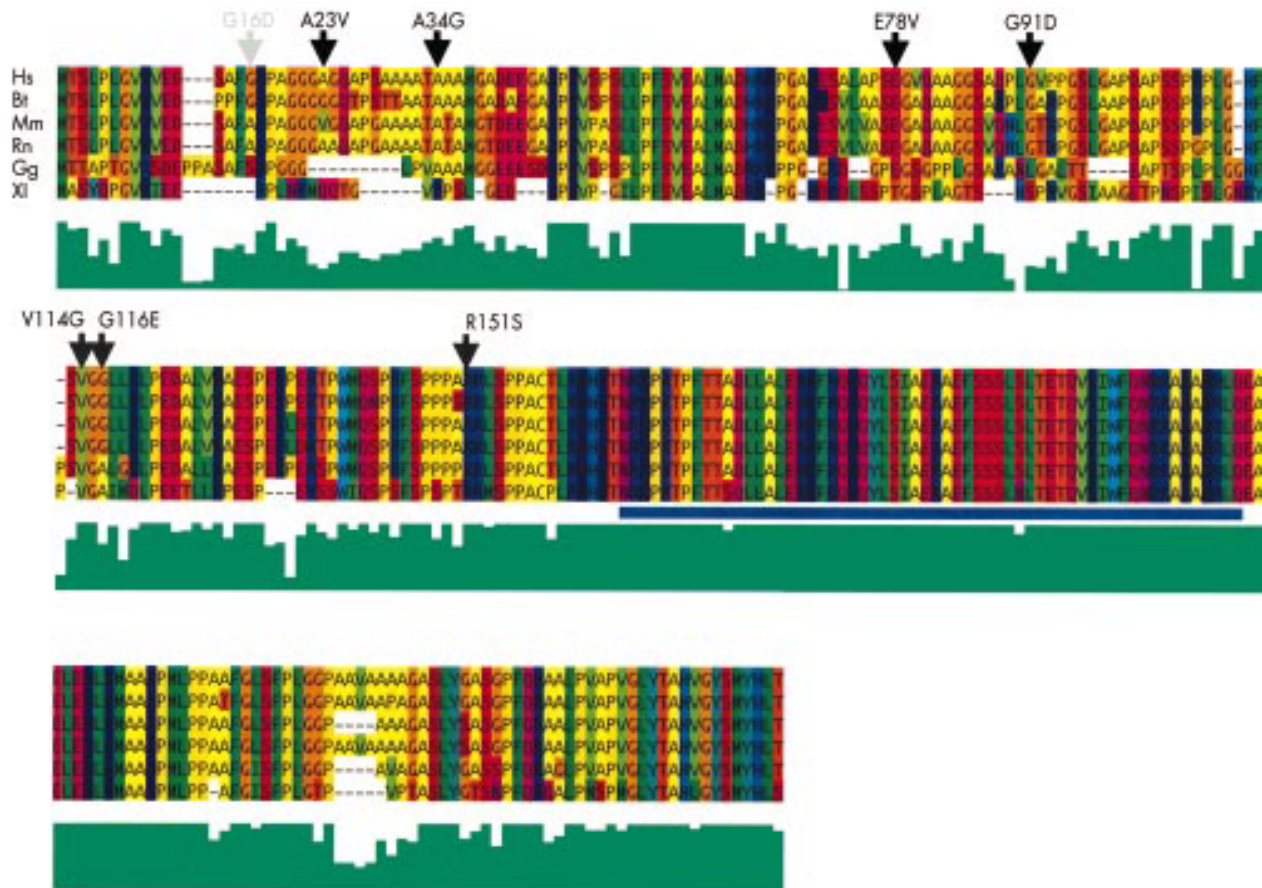
Figure 2 Protein sequence alignment for MSX1 . The human MSX1 sequence is aligned with the B taurus , M musculus , R norvegicus , G gallus , and X laevis sequence using ClustalW. Non-conserved amino acid variants from controls (grey) and cases (black) are indicated with arrows above the appropriate residue. The green bar graph below each position is a quantitative ClustalW function to show the degree of sequence homology. The homeobox region is underlined by a blue bar.
