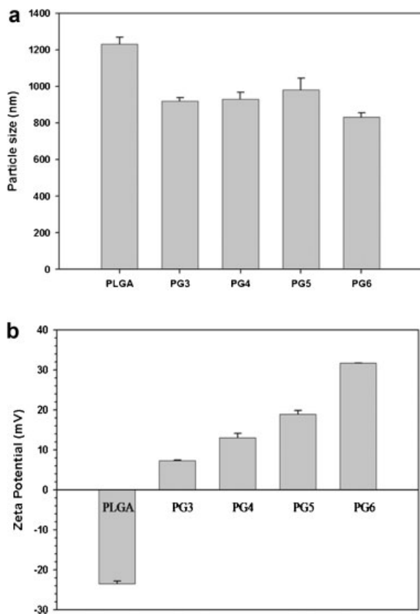
Figure 4. Particle size and zeta potential of PLGA microparticles loaded with PAMAM-pDNA dendriplexes (PG3-PG6). Particle size (a) and zeta potential (b) of PLGA microparticles loaded with PAMAM-pDNA dendriplexes. Data are represented as the mean \pm standard deviation ( n = 3 ).
